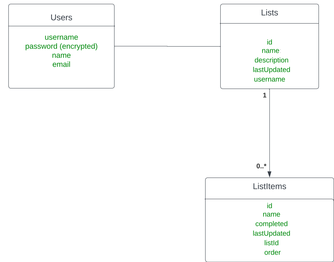
Database SQL Diagram
